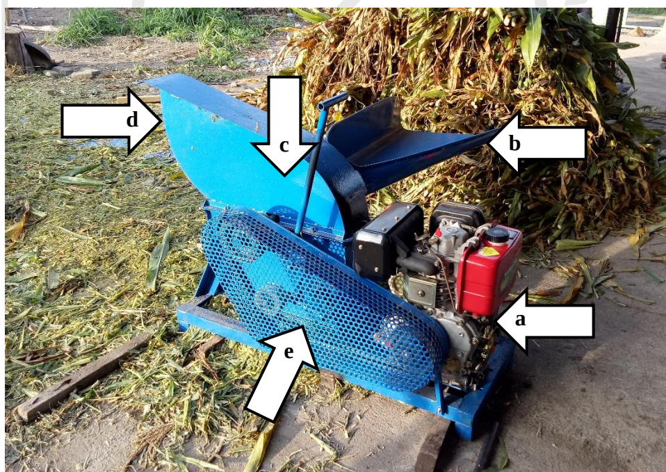
Figure 1. Parts of EXCELHIGH FC-2A Forage Chopper powered by 7.46 kW YAMADA 186F Diesel Engine: (a) Prime mover, (b) Feeding table, (c) Chopping chamber, (d) Output chute, and (e) Belt and pulley transmission system with cover.
